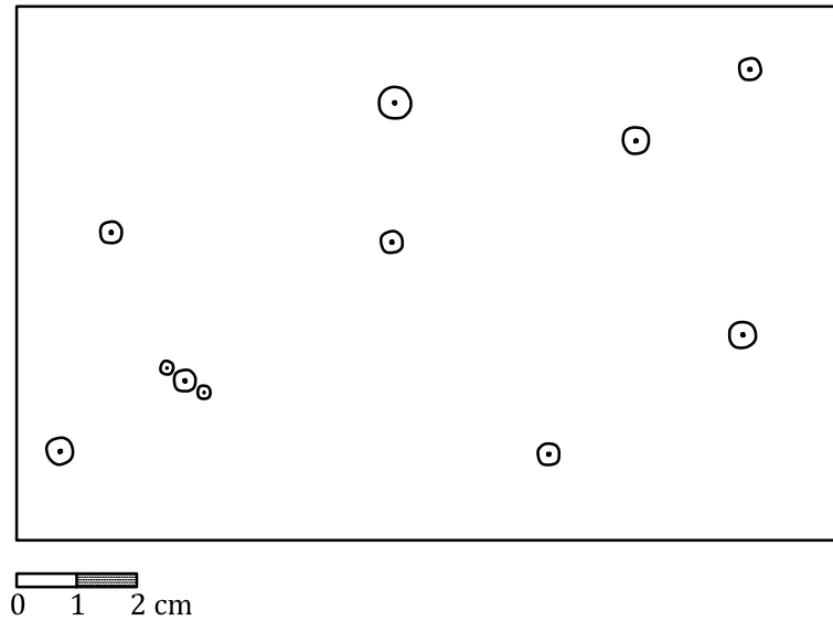
Figure A.5 — Shape and location of marks — Class D
